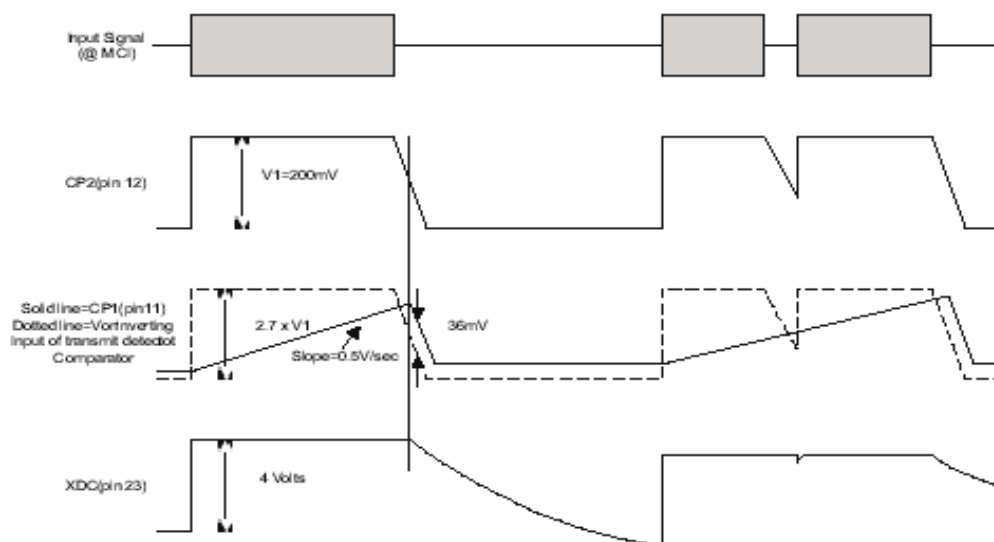
Fig 10 Response At CP1 and CP2
