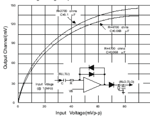
Fig 8 Log Amp Transfer Characteristics
