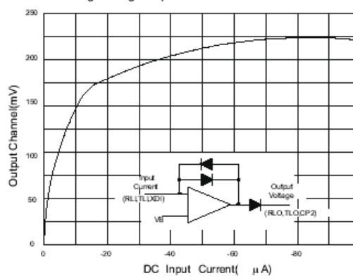
Fig 7 Log Amp Transfer Characteristics
