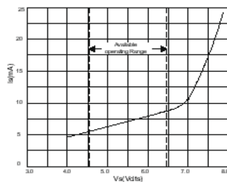
Fig 15 Supply Current vs Supply Voltage
