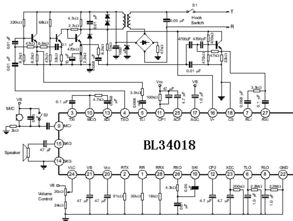
Fig 16 basic Line powered Speakerphone
