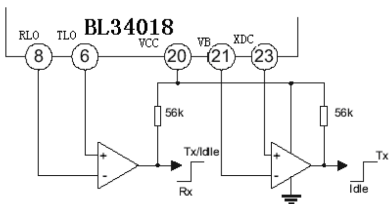
Fig 17 Digital Transmit/Idle/Receive Indication
