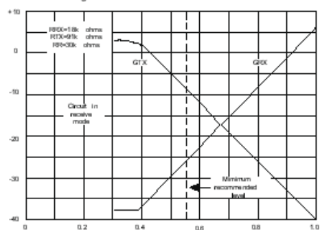
Fig 5 Attenuation Gain versus VLC
