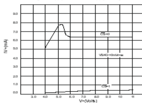
Fig 12 Supply Current vs Supply Voltage
