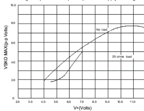
Fig 9 Speaker Amp Output vs Supply Voltage
