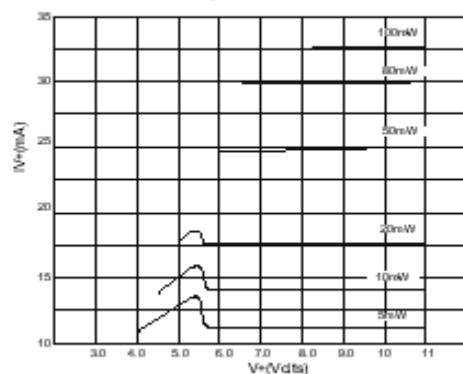
Fig 13 Supply Current vs Supply Voltage vs Speaker Power
