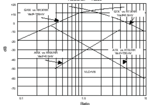
Fig 4 Gain and attenuation versus Resistor Ratio
