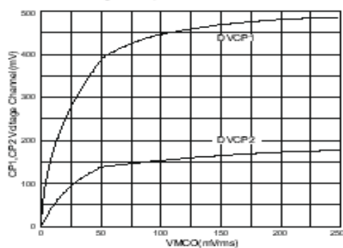
Fig 10 Response At CP1 and CP2
