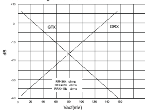
Fig 6 Attenuator Gain vs Vacf
