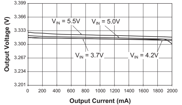
DC Regulation
