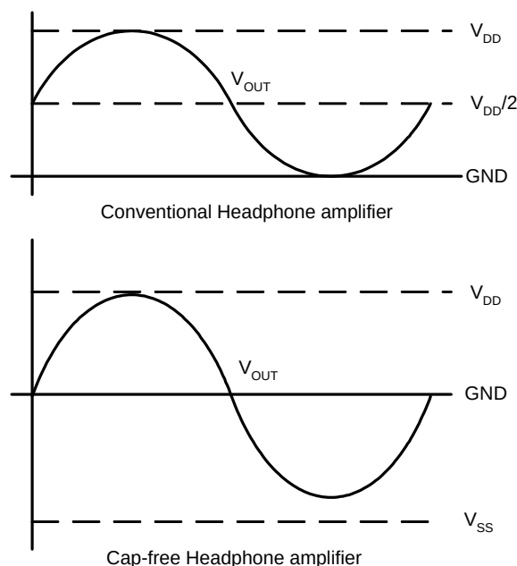
Figure 1. Cap-Free Operation
