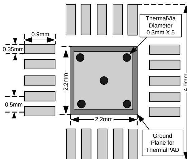
Figure 2. TQFN4x4-20B Layout Recommendation
