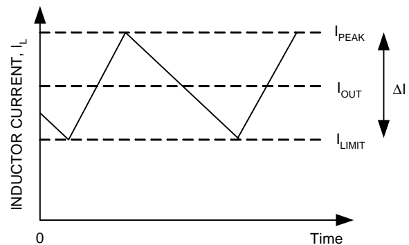
Figure 2. Current-Limit Algorithm
