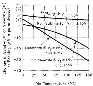
EL4422, EL4442, and EL4444 Bandwidth, Slewrate, and Peaking vs. Temperature, Av = +2, RL = 150Ω, RL = 270Ω, CF = 3 pF
