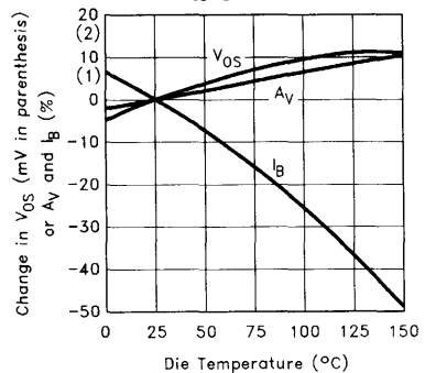
Change in V_{OS} , I_B , and A_V vs. Temperature
