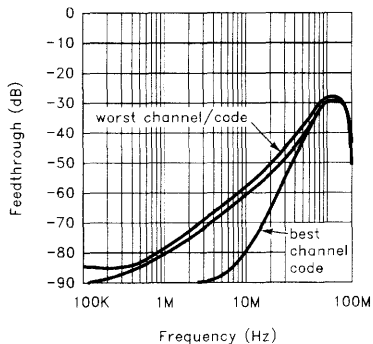
EL4421, EL4441, and EL4443 Unselected Channel Feedthrough vs. Frequency
