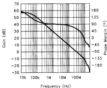
EL4443 Open-Loop Gain and Phase vs. Frequency
