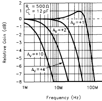
EL4421, EL4441, and EL4443 Frequency Response for Various Gains
