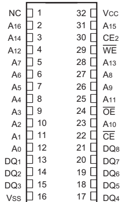
32-pin Ceramic LCC
