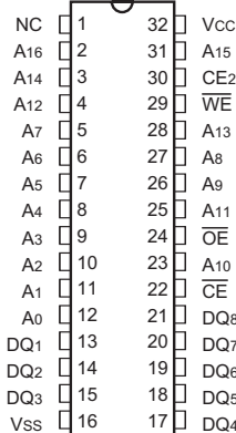
32-pin Ceramic DIP 32-pin Ceramic SOJ
