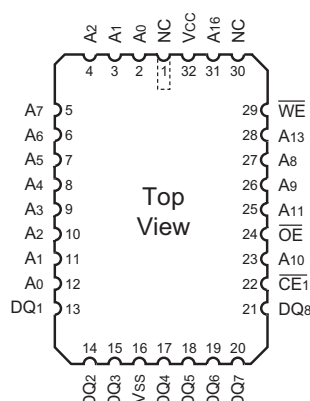
32-pin Quad CLCC
