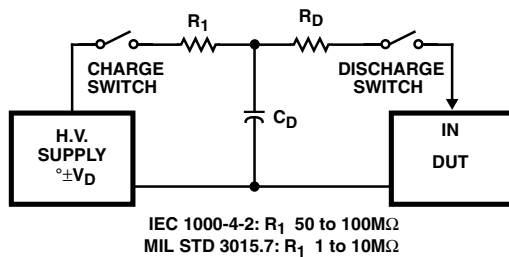
FIGURE 1. ELECTROSTATIC DISCHARGE TEST
