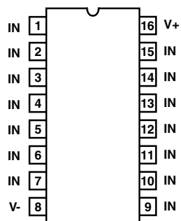
SP720MD (SBDIP) TOP VIEW
