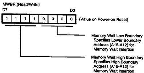
Figure 27. Memory Wait Boundary Register
