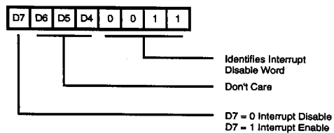
Figure 14. Interrupt Disable Word
