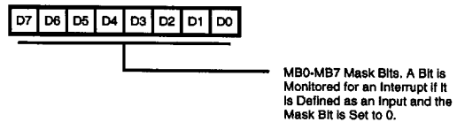
Figure 13. Mask Control Word
