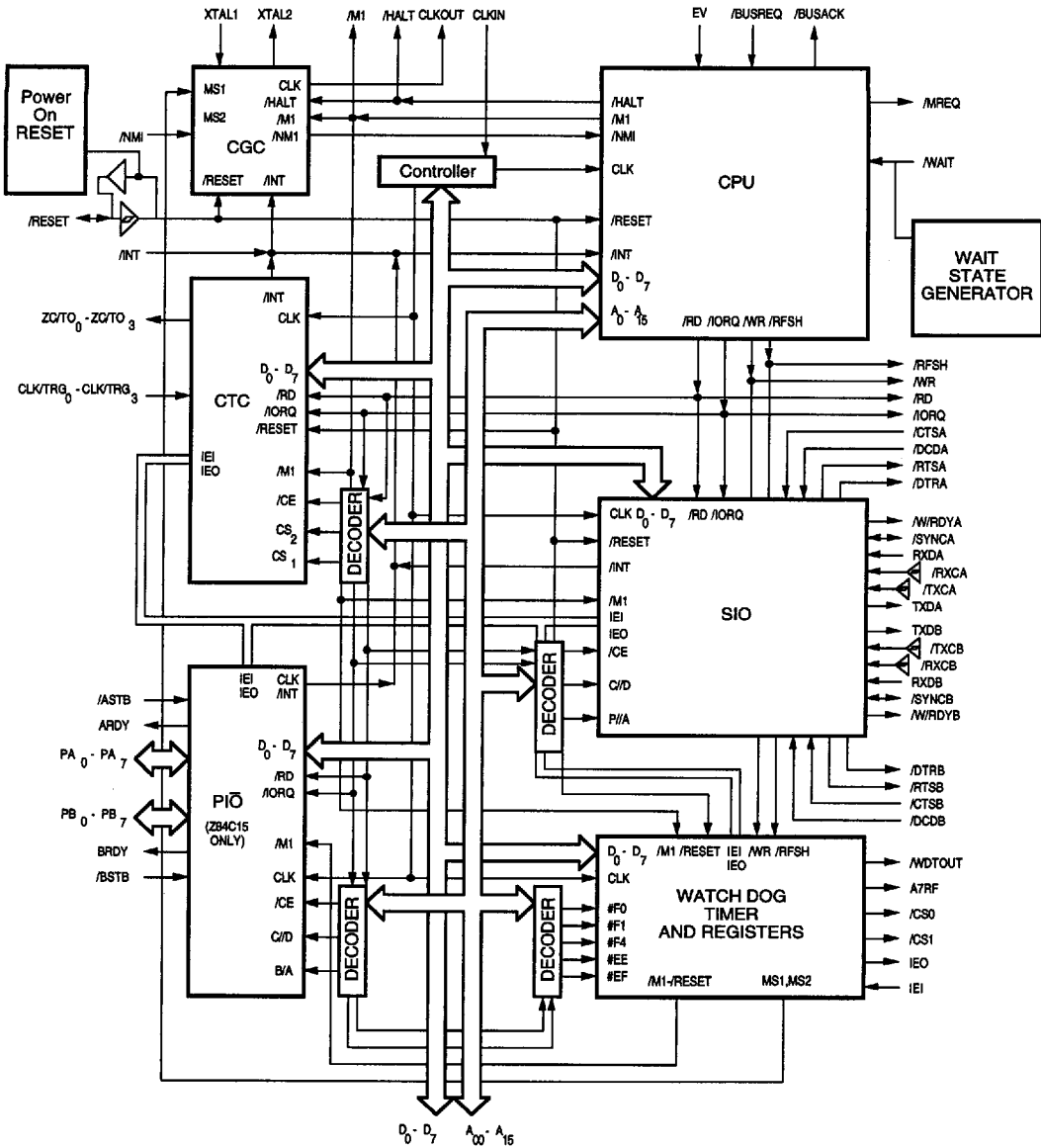
Figure 3(b). Block Diagram for Z84C15 IPC
