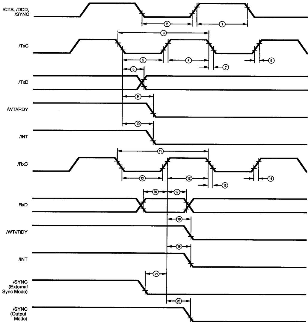
Figure 56. SIO Timing (See Table F)
