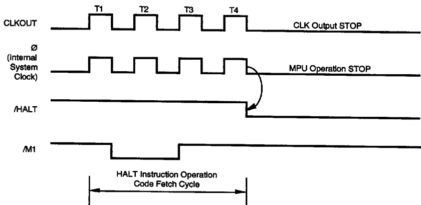
Figure 33. STOP Mode Timing (At Halt Instruction Execution)
