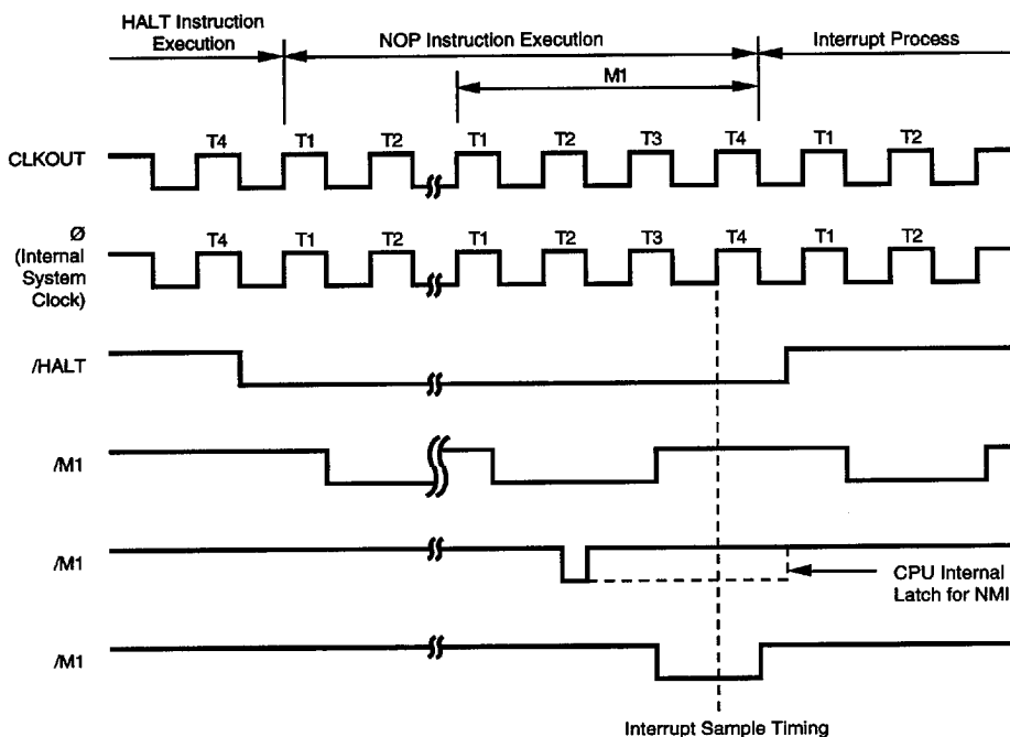
Figure 34. Halt Release Operation Timing By Interrupt Request Signal in RUN Mode
