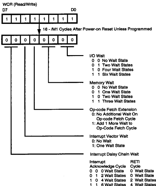
Figure 26. Wait State Control Register
