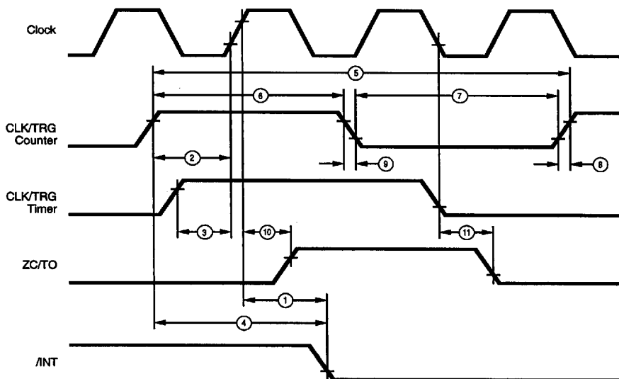
Figure 55. Counter/Timer Timing (See Table E)
