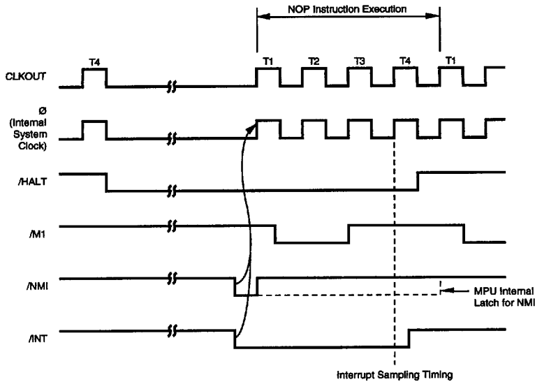
(a) IDLE1 Mode
