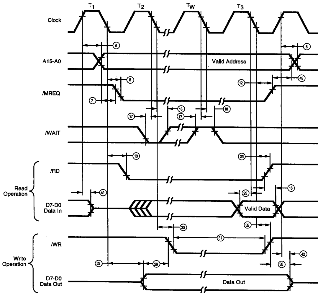
Figure 41. Memory Read or Write Cycle (See Table A)
