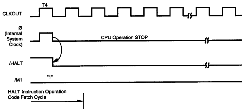
Figure 32. IDLE2 Mode Timing (At Halt Instruction Execution)
