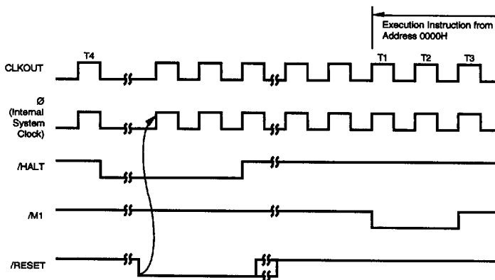
(a) IDLE1 Mode
