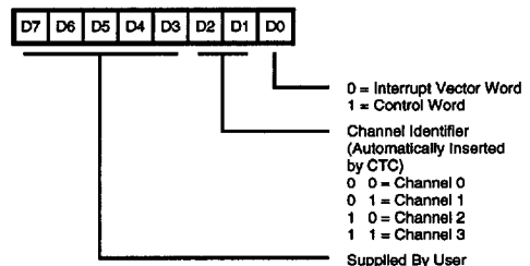
Figure 17. CTC Interrupt Vector Word
