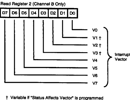
Figure 18c. SIO Read Register 2
