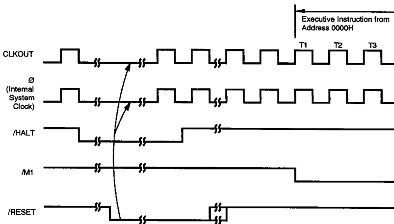
Figure 39. Halt Release Operation Timing By Reset in STOP Mode
