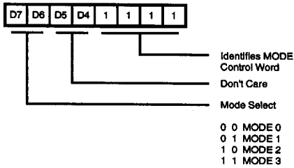
Figure 10. PIO Mode Control Word
