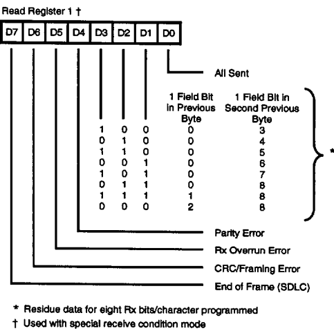
Figure 18b. SIO Read Register 1
