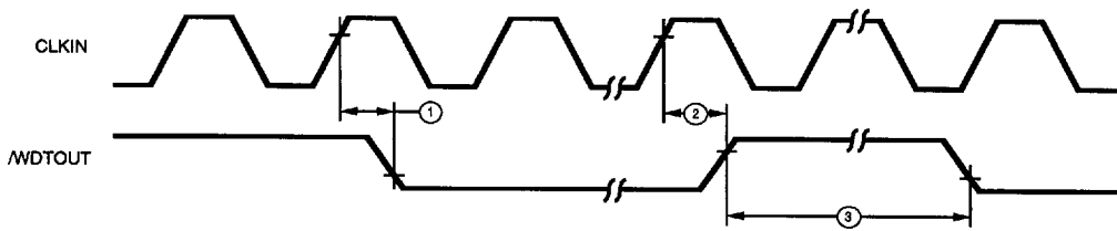
Figure 57. Watch-Dog Timer Timing (See Table H)
