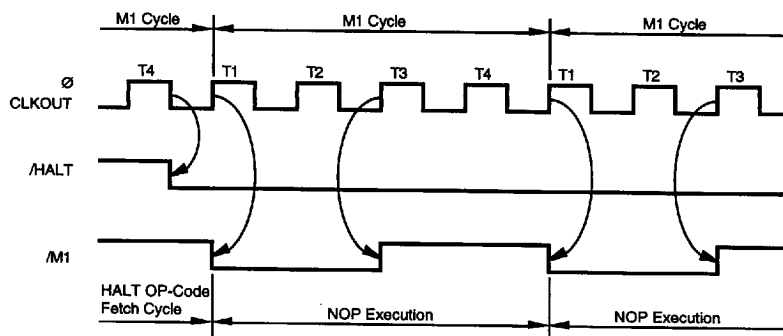
Figure 30. Timing of RUN Mode (at Halt Instruction Command Execution)
