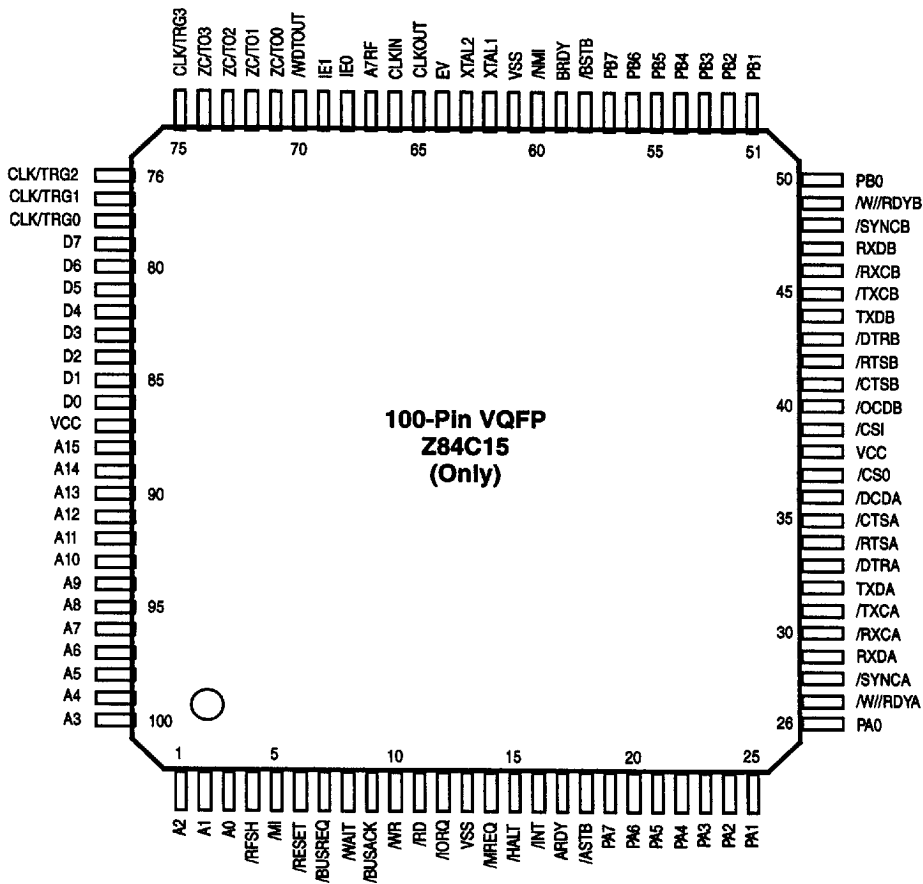
Figure 2. Z84C15 Pin Assignments
