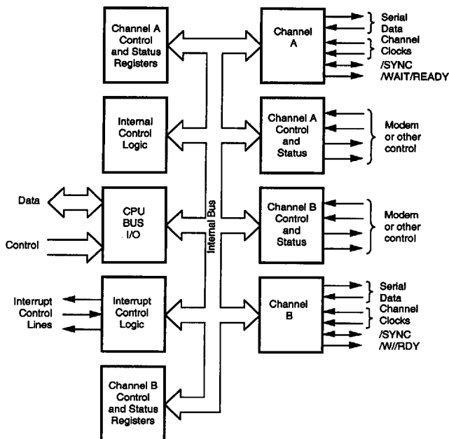
Figure 6. SIO Block Diagram
