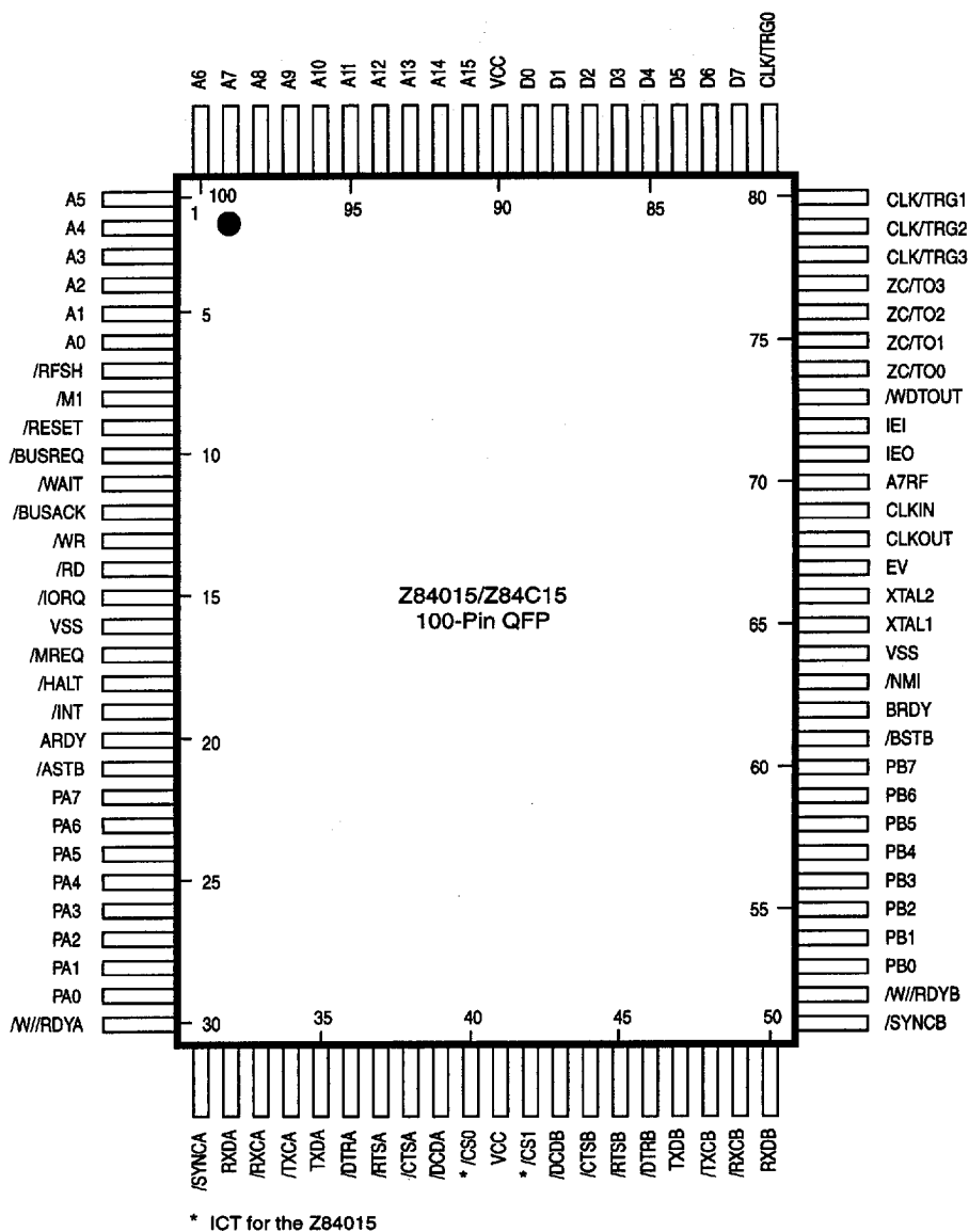
Figure 1. Z84015/C15 Pin Assignments
