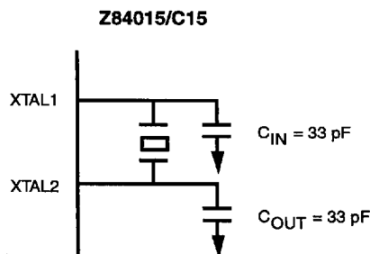
Figure 8. Circuit Configuration For Crystal
