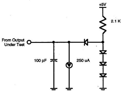
Figure 58. Standard Test Load
