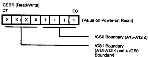
Figure 28. Chip Select Boundary Register
