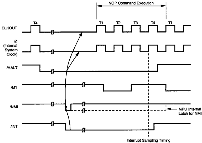
Figure 38. Halt Release Operation Timing By Interrupt Request Signal in STOP Mode
