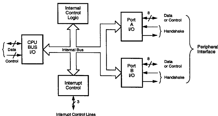
Figure 4. PIO Block Diagram
