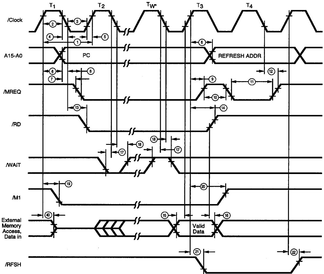
Figure 40. Instruction Op-code Fetch (See Table A)
