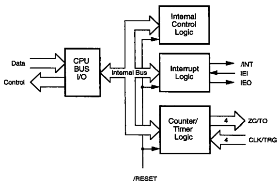
Figure 5. CTC Block Diagram
