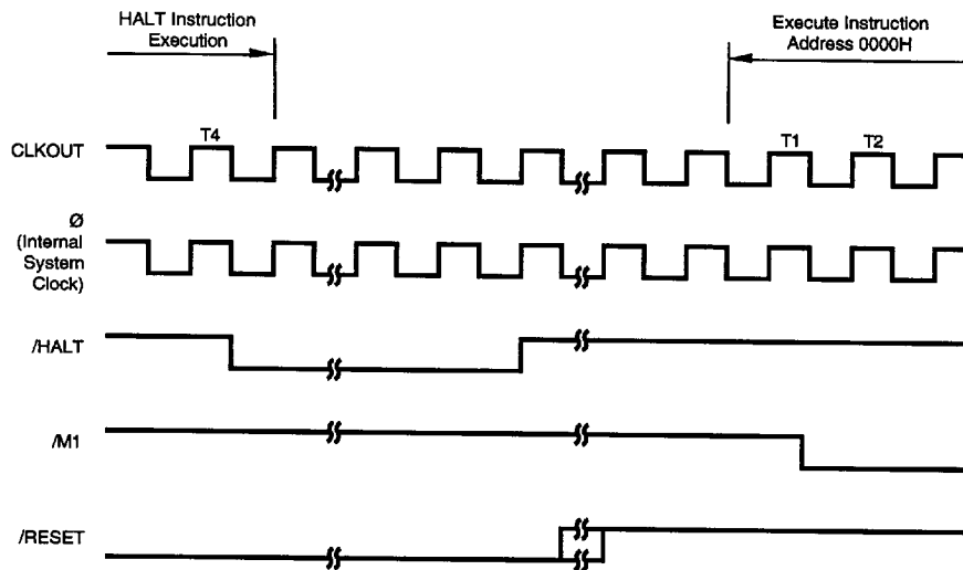
Figure 35. Halt Release Operation Timing By Reset in RUN Mode
