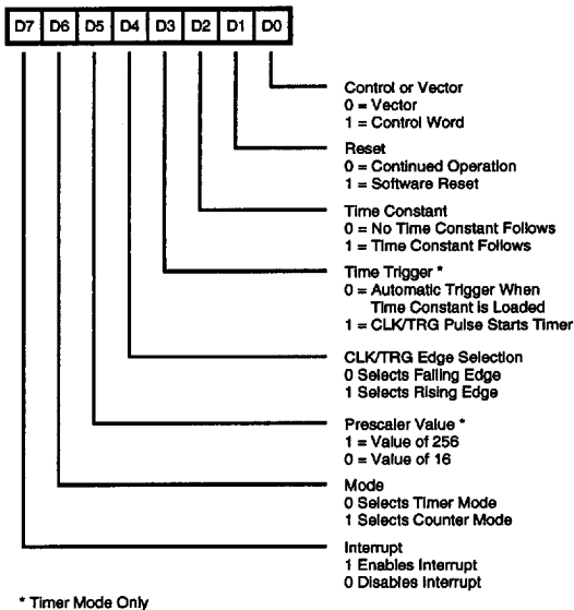
Figure 15. CTC Channel Control Word
