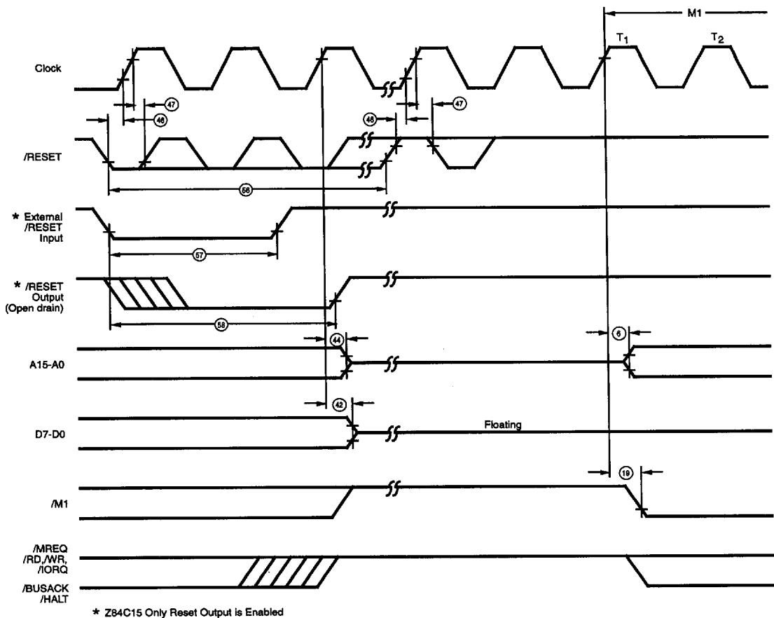
Figure 47. Reset Cycle (See Table A)
