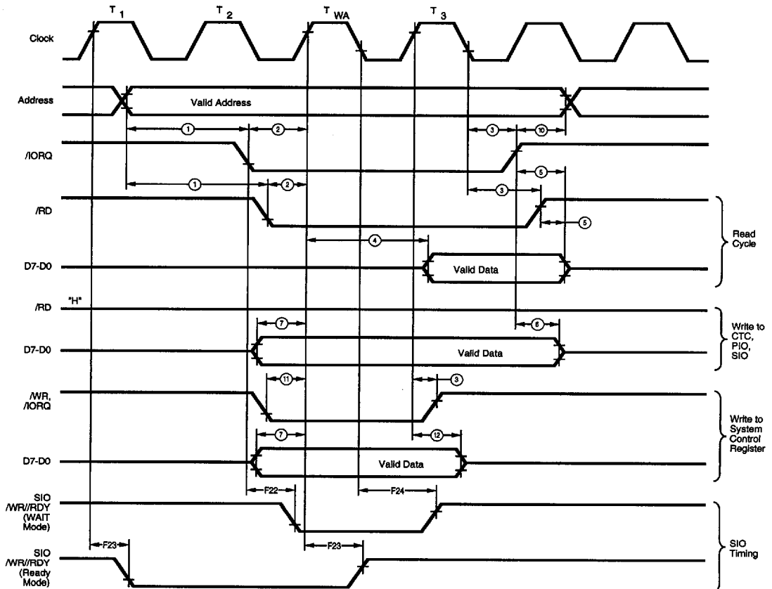
(a) On-chip peripheral I/O access from External Bus master (See Tables C and F)
