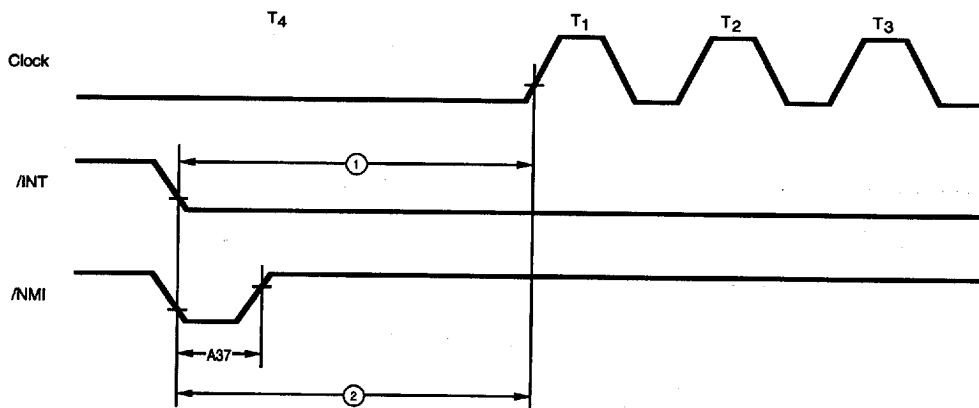
Figure 49. Clock Restart Timing by /INT, /NMI (STOP Mode) (See Table B)
