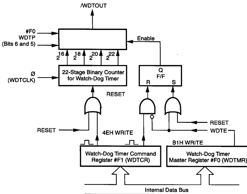
Figure 7. Block Diagram of Watch-Dog Timer
