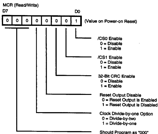
Figure 29. Misc. Control Register
