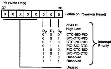
Figure 23. Interrupt Priority Register
