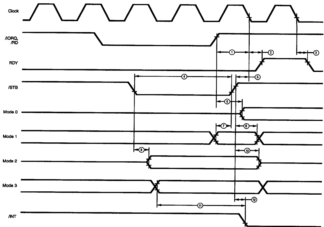
Figure 54. PIO Timing (See Table D)
