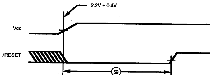
Figure 48. Reset on Power-up (Applies only for Z84C15) (See Table B)
