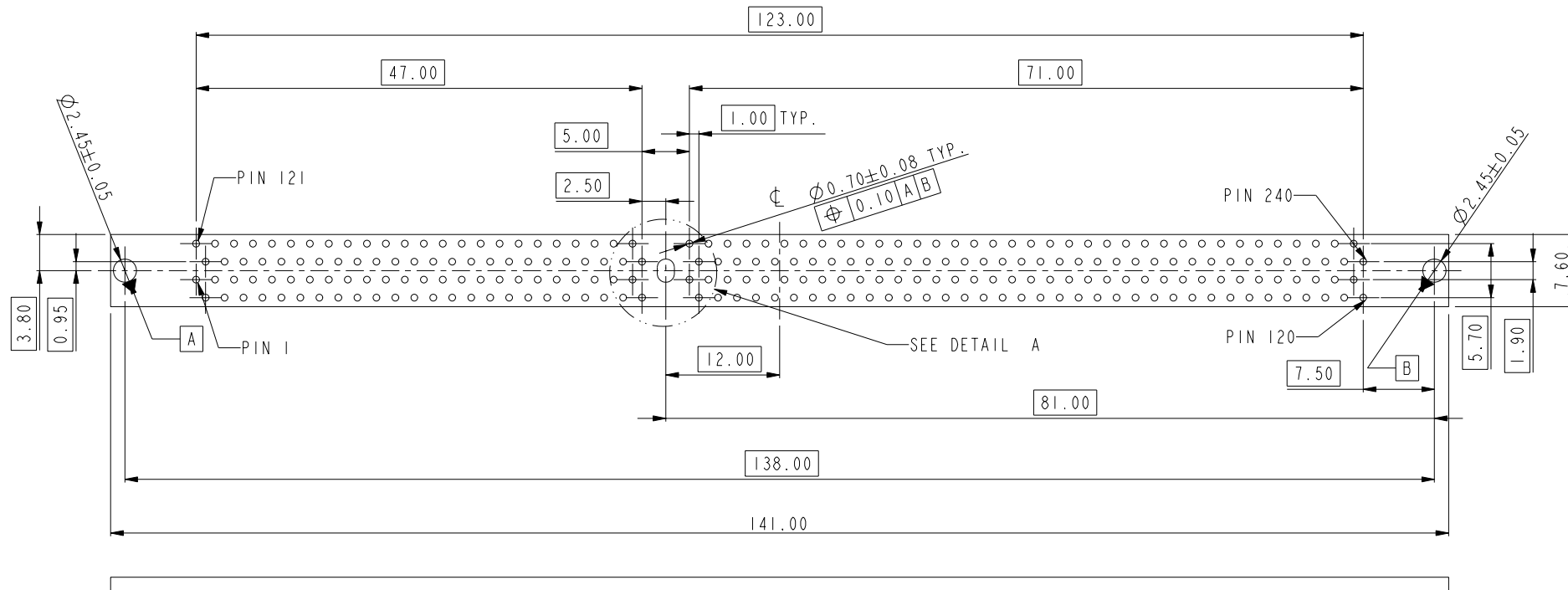
RECOMMENDED CIRCUIT BOARD HOLE LAYOUT
