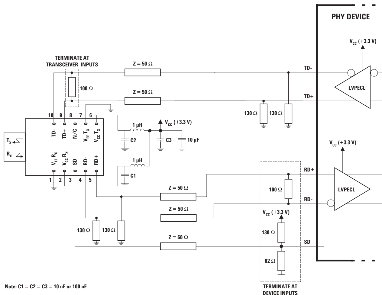
Figure 4. Recommended Decoupling and Termination Circuits
