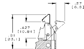
SHORT LATCH EJECTOR for IDS2 without strain relief
