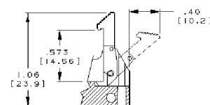
LONG LATCH EJECTOR for IDS2 with strain relief
