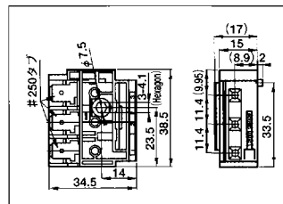
TERMINAL CONNECTOR BOARD 端子台コネクタ
