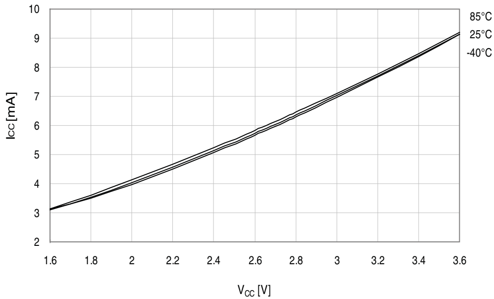
Figure 36-7. Active mode supply current vs. V_{CC} .
