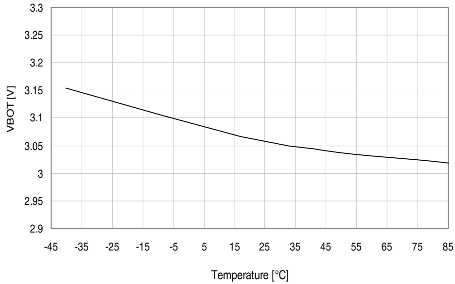
Figure 36-47. BOD thresholds vs. temperature.
