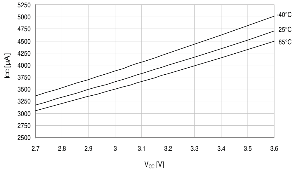
Figure 36-14. Idle mode current vs. V_{CC} .
