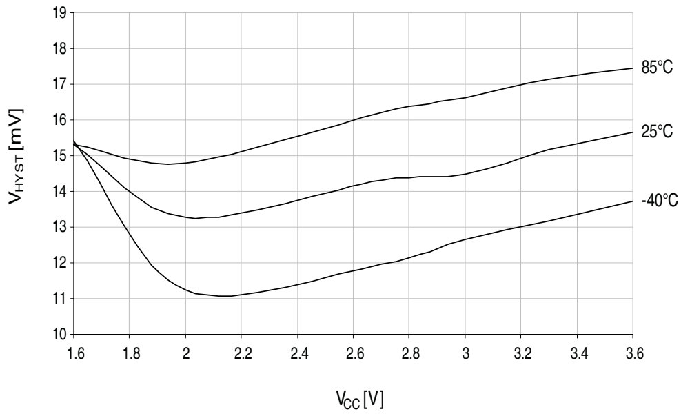
Figure 36-42. Analog comparator hysteresis vs. V_{CC} . Large hysteresis.
