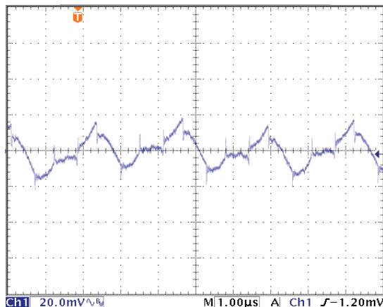
Output Ripple & Noise ( V_{IN} = 12V , I_{OUT} = 20A , C_{OUT} = 10\mu F \parallel 1\mu F , scope = 20 MHz BW) Vertical = 20 mV/div., Sweep = 1 \mu S/div.
