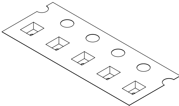
Figure 22. Emitter pocket tape packaging for Blue, Green, Royal-Blue and Cyan.
