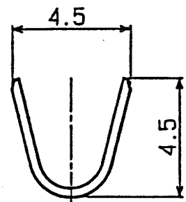
B-B SEC.
