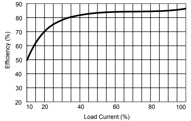
Figure 4: Efficiency vs. Output Load (Dual Output)
