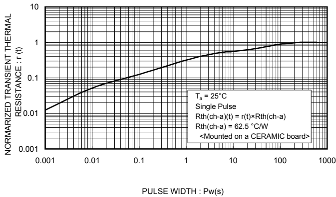
Fig. 15 Normalized Transient Thermal Resistance vs. Pulse Width
