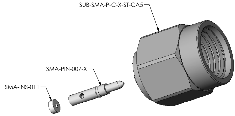
FIG.1 SMA-P-C-X-ST-CA5 SHOWN
