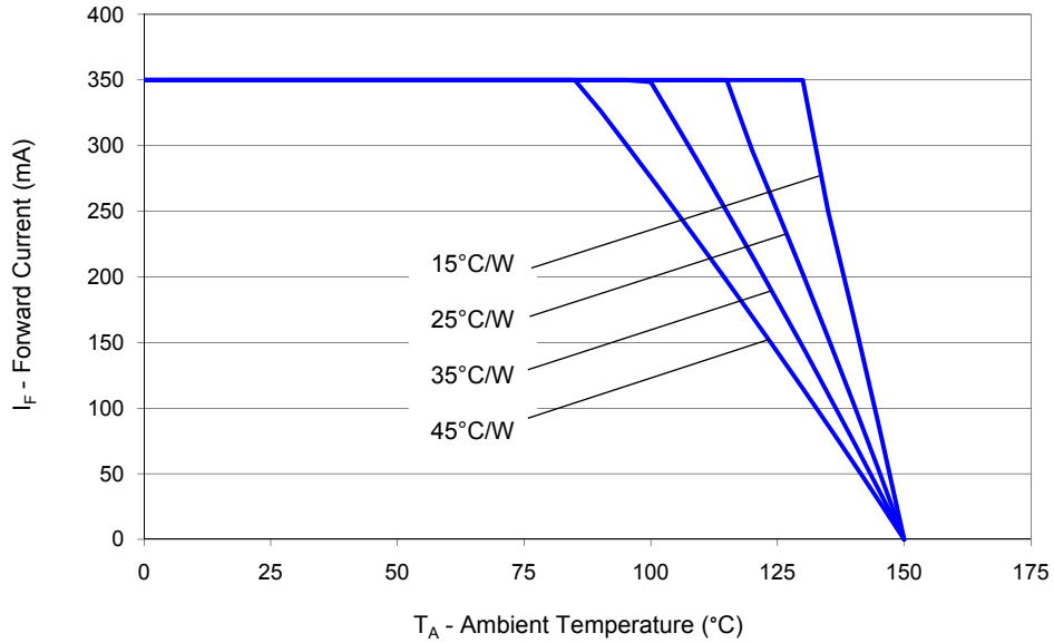
Figure 19. Maximum forward current vs. ambient temperature, based on T_{JMAX} = 150^{\circ}C .
