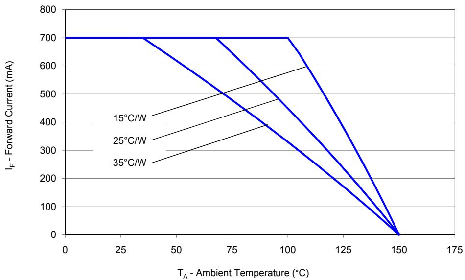
Figure 20. Maximum forward current vs. ambient temperature, based on T_{JMAX} = 150^{\circ}C .
