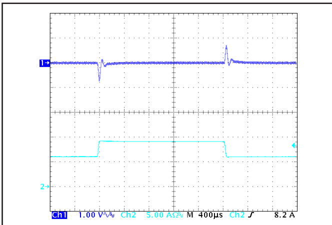
Figure 5: Output voltage response to step-change in load current (50%-75%-50% of Iout(max)); di/dt = 0.1 \text{ A}/\mu\text{s} . Load cap: 1 µF ceramic capacitor. Ch 1: Vout (1 V/div), Ch 2: Iout (5 A/div).
