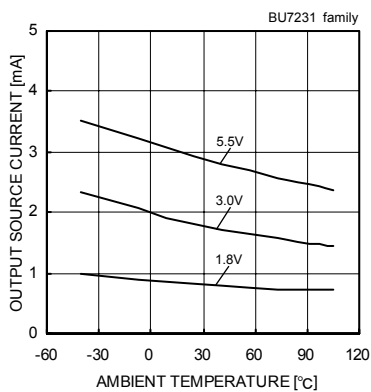
Fig.10 Output Source Current - Ambient Temperature (VOU=VDD-0.4[V])
