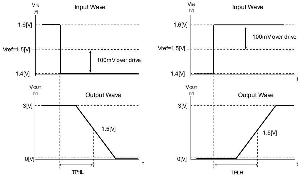
Fig4. Slew rate
