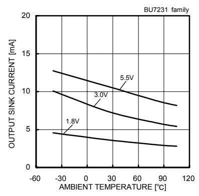
Fig.12 Output Sink Current - Ambient Temperature (VOU=VSS+0.4[V])
