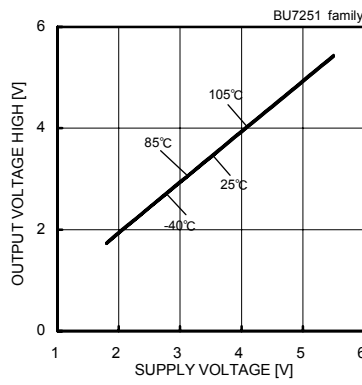
Fig.5 Output Voltage High - Supply Voltage (RL=10[kΩ])
