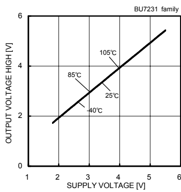
Fig.5 Output Voltage - Supply Voltage (RL=10[kΩ])
