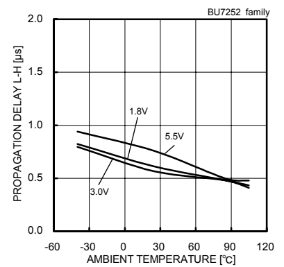
Fig. 21 Propagation Delay L-H – Ambient Temperature
