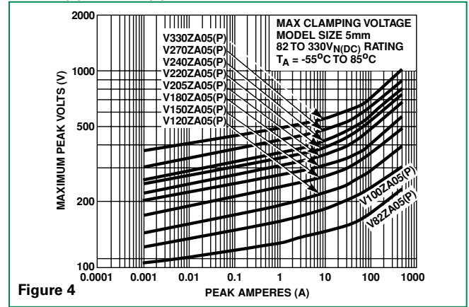
V82ZA05(P) - V330ZA05(P)
