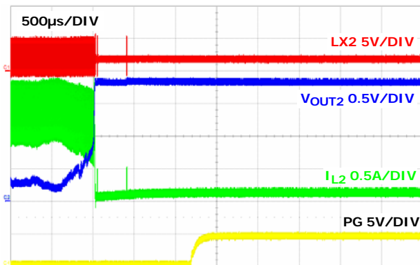
FIGURE 41. OUTPUT SHORT CIRCUIT RECOVERY CHANNEL 2
