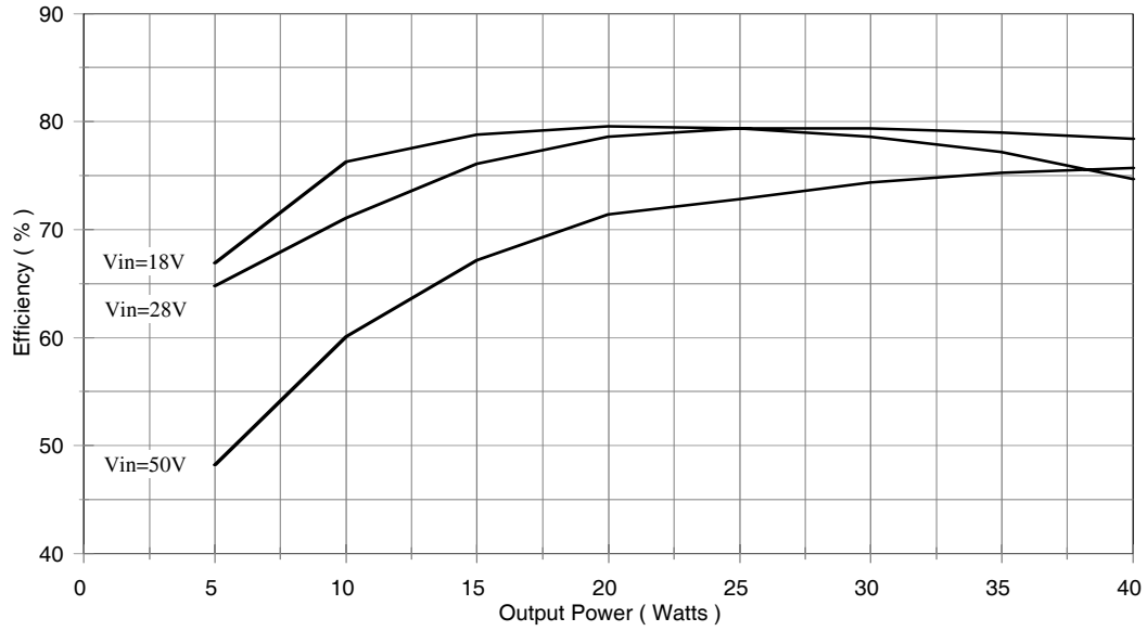
Figure 5. M3G280515T Efficiency vs Line and Load
