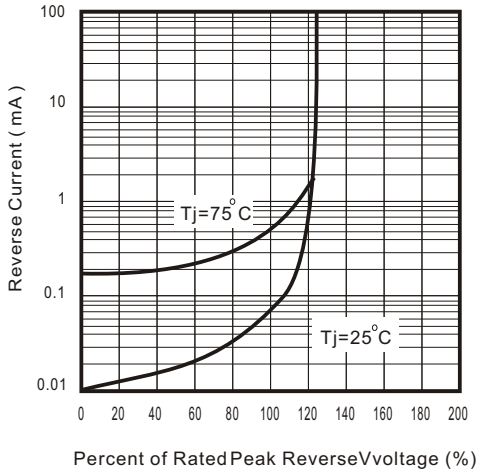
Fig. 1 - Reverse Characteristics
