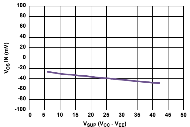
FIGURE 14. V_{OS IN} vs SUPPLY VOLTAGE ( V_{CC} - V_{EE} )
