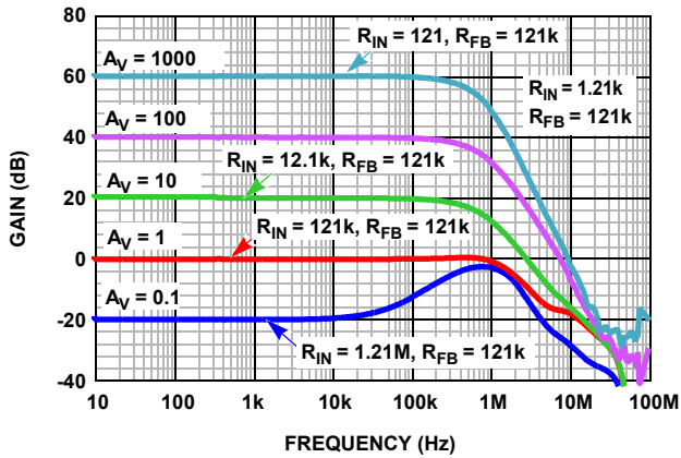
FIGURE 19. CLOSED LOOP GAIN ( R_{FB} = 121k ) vs FREQUENCY
