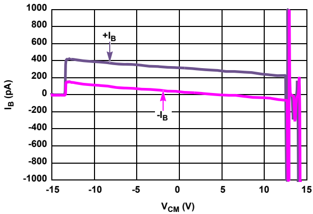
FIGURE 11. I_B vs INPUT COMMON MODE VOLTAGE
