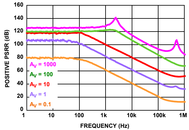
FIGURE 22. POSITIVE PSRR V_{EE} AND V_{CC} ( R_F = 121k )
