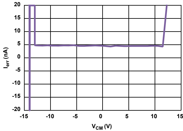
FIGURE 5. I_{ERR} vs INPUT COMMON MODE VOLTAGE
