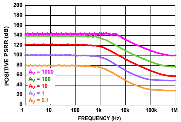
FIGURE 26. POSITIVE PSRR V_{EO} AND V_{CO} ( R_F = 121k )
