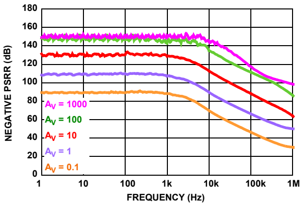
FIGURE 25. NEGATIVE PSRR V_{EO} AND V_{CO} ( R_F = 30.1k )
