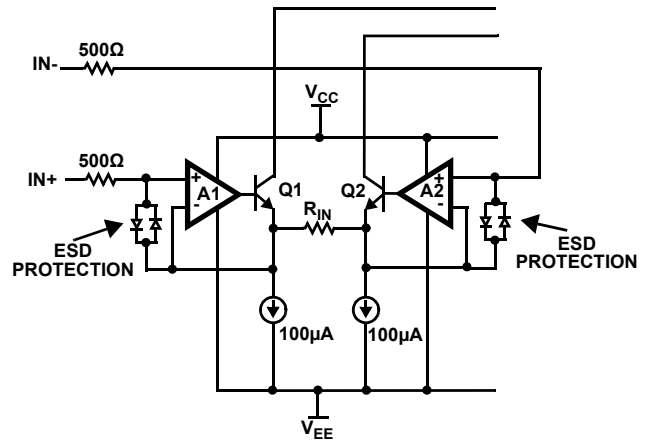
FIGURE 33. INPUT STAGE ESD PROTECTION DIODES
