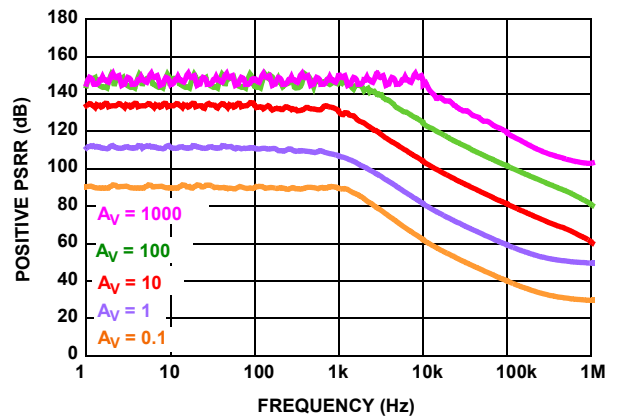
FIGURE 24. POSITIVE PSRR V_{EO} AND V_{CO} ( R_F = 30.1k )
