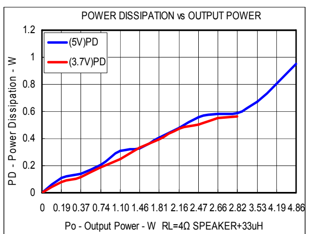
Dissipation vs. Output Power (40hm)
