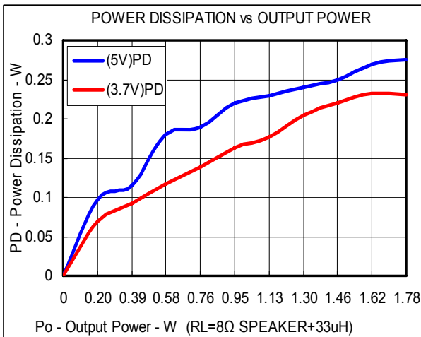
Dissipation vs. Output Power (80hm)
