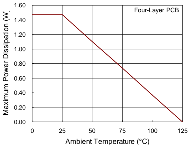
Figure 2. Derating Curve for RT8510 Package
