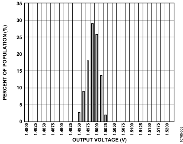
Figure 3. X-Axis Zero g Output Voltage at 25°C, V_S = 3 V
