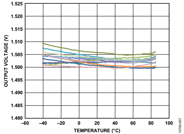
Figure 7. Y-Axis Zero g Offset vs. Temperature, V_S = 3 V (14 Parts Soldered to PCB)
