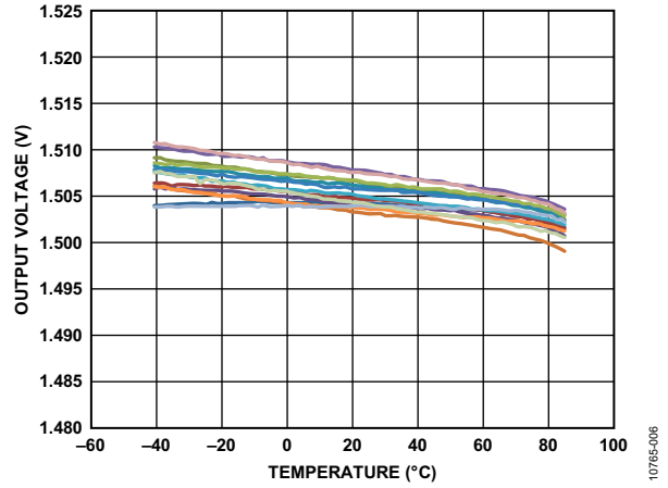
Figure 6. X-Axis Zero g Offset vs. Temperature, V_S = 3 V (14 Parts Soldered to PCB)
