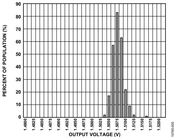
Figure 5. Z-Axis One g Output Voltage at 25°C, V_S = 3 V
