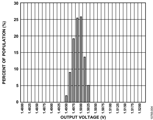
Figure 4. Y-Axis Zero g Output Voltage at 25°C, V_S = 3 V
