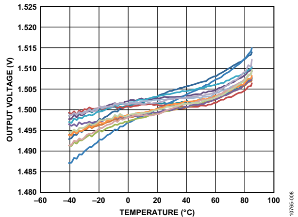
Figure 8. Z-Axis Zero g Offset vs. Temperature, V_S = 3 V (14 Parts Soldered to PCB)
