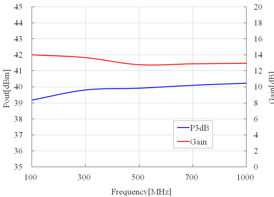
P3dB & Gain vs. Frequency
