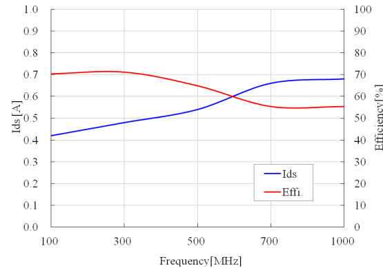
Ids & Efficiency vs. Frequency (@ P3dB)
