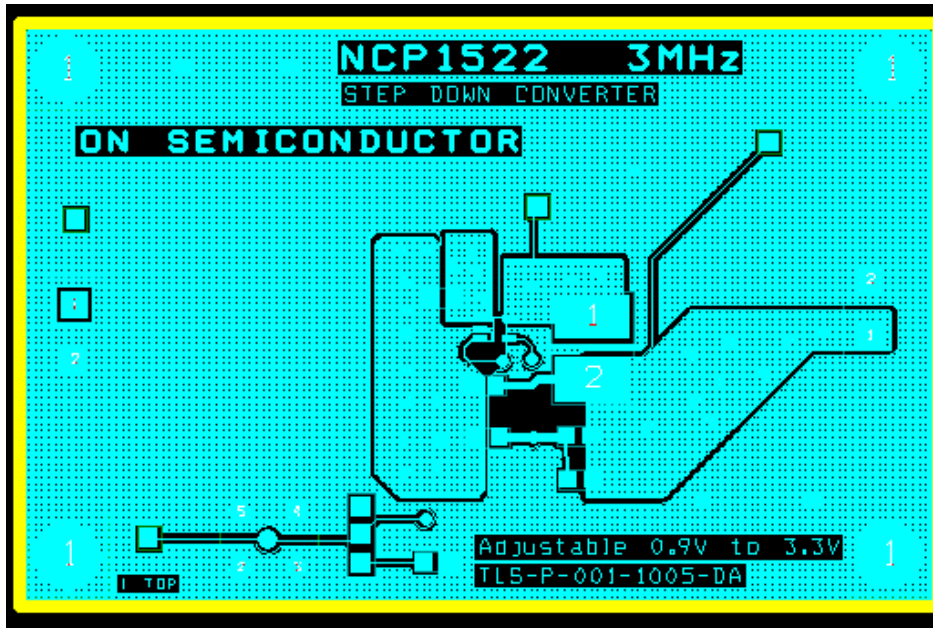
Figure 29. Board Layout (Top View)
