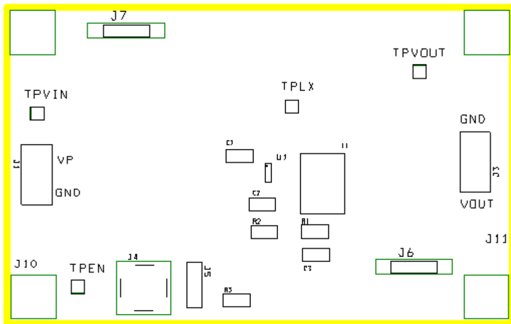
Figure 28. Silkscreen Layer
