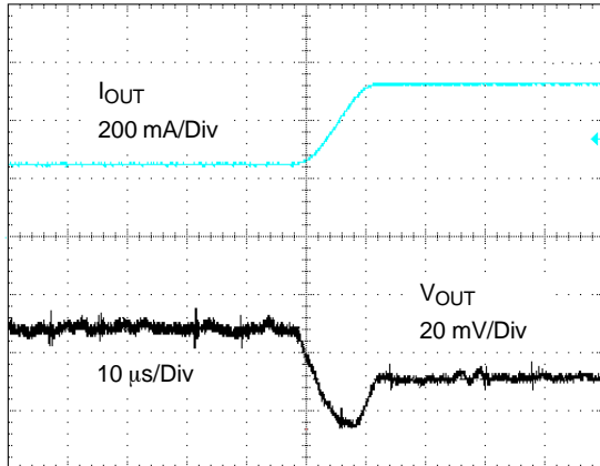
Figure 19. Load Transient Response in PWM Operation ( V_{IN} = 3.6 V)
