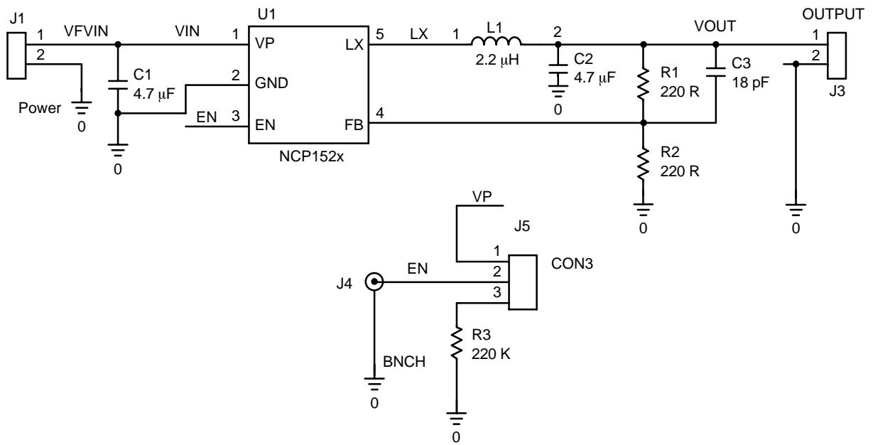
Figure 27. Schematics
