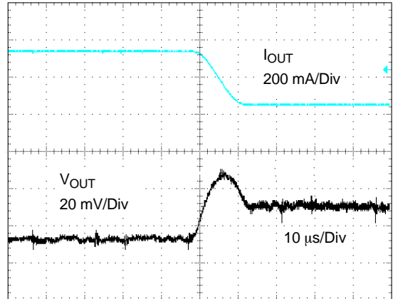
Figure 20. Load Transient Response in PWM Operation ( V_{IN} = 3.6 V)
