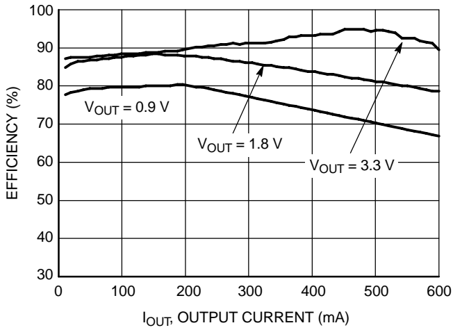
Figure 10. Efficiency vs. Output Current (V IN = 4.0 V)
