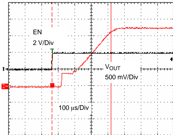
Figure 21. Soft Start Time ( V_{IN} = 3.6 V)
