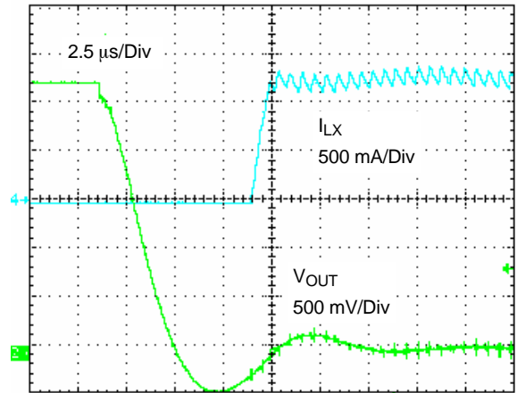
Figure 22. Short Circuit Protection ( V_{IN} = 3.6 V)
