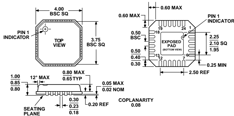
Figure 34. 24-Lead Lead Frame Chip Scale Package [LFCSP] 4 mm × 4 mm Body (CP-24) Dimensions shown in millimeters
