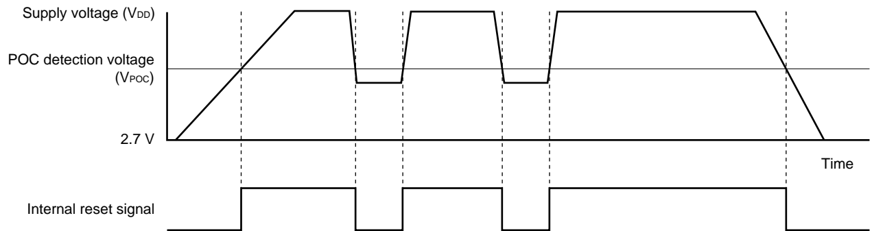
Figure 24-2. Timing of Internal Reset Signal Generation in Power-on-Clear Circuit
