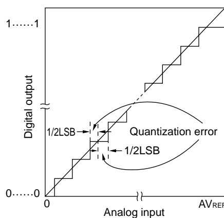
Figure 13-13. Quantization Error
