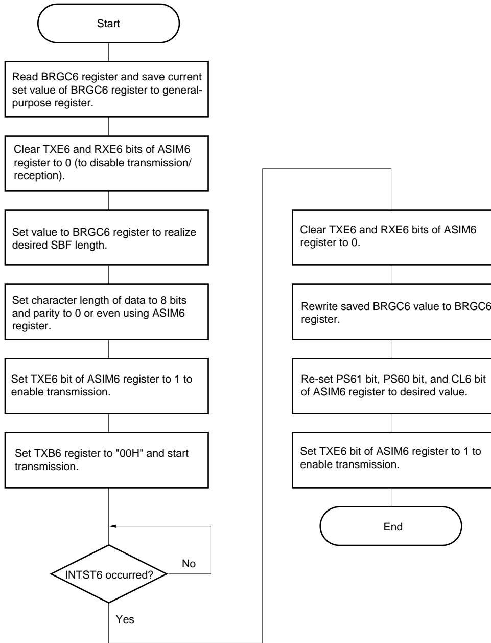
Figure 15-23. SBF Transmission
