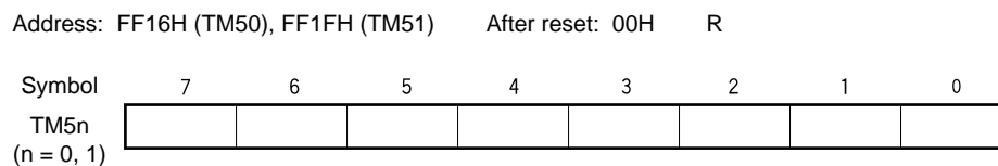
★ Figure 8-3. Format of 8-Bit Timer Counter 5n (TM5n)
