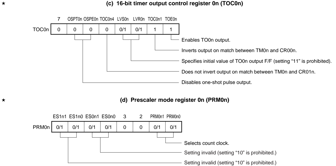
Figure 7-34. Control Register Settings in Square-Wave Output Mode (2/2)
