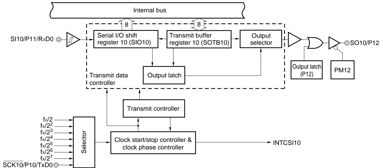
Figure 16-1. Block Diagram of Serial Interface CSI10
