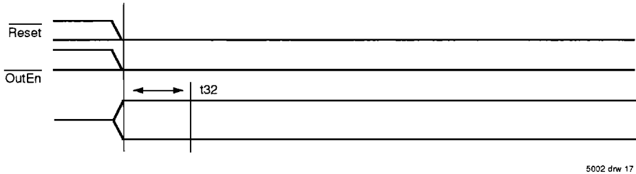
Figure 15. Reset Timing for Access Type Out
