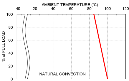
PDS02-48S05W Derating Curve
