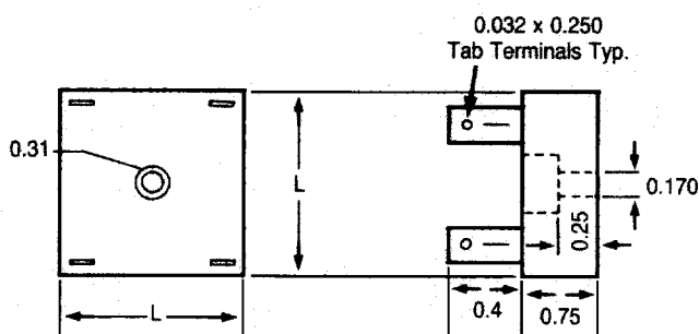
Figure 23—High Voltage Bridge
