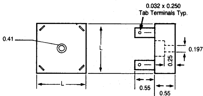
Figure 22—High Voltage Bridge
