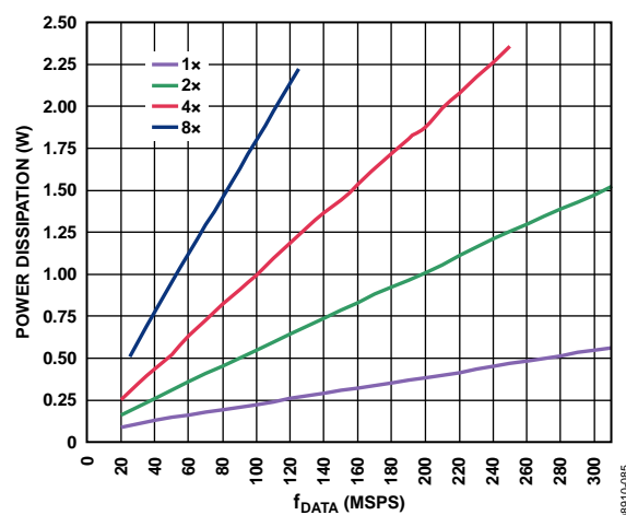
Figure 86. DVDD18 Power Dissipation vs. f_{\text{DATA}} with Fine Modulation, PLL, and Inverse Sinc Filter Disabled
