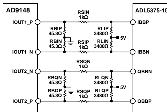
Figure 81. Passive Level Shifting Network for Biasing the ADL5375-15 from the AD9148
