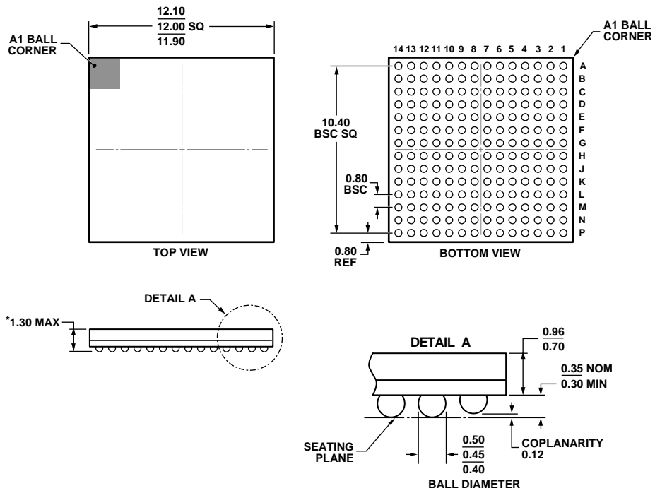
Figure 94. 196-Ball Chip Scale Package, Ball Grid Array [CSP_BGA] BC-196-7 Dimensions shown in millimeters
