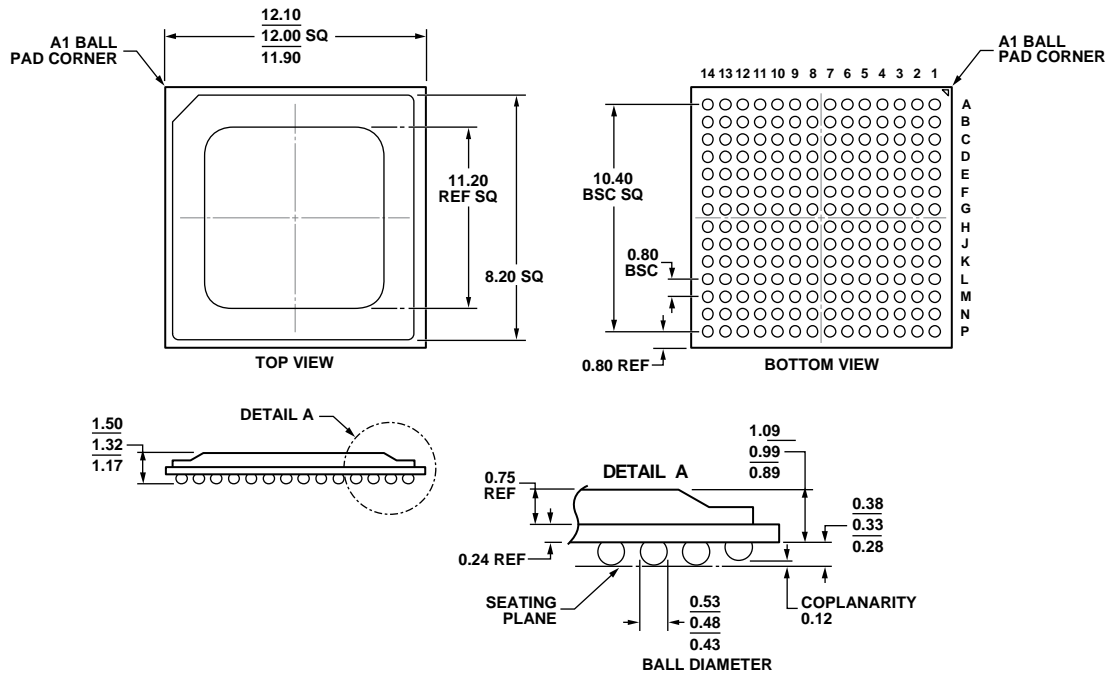
Figure 95. 196-Ball Ball Grid Array, Thermally Enhanced [BGA_ED] BP-196-1 Dimensions shown in millimeters
