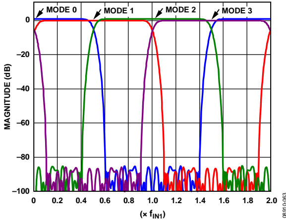
Figure 63. HB1 Filter Modes
