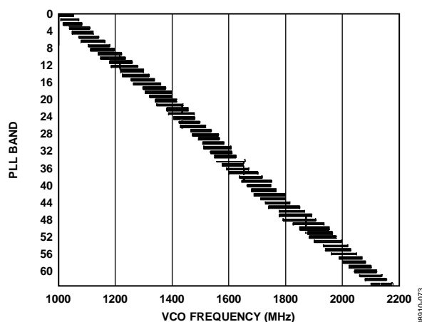
Figure 74. PLL Lock Range Overtemperature for a Typical Device
