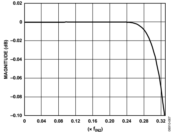
Figure 67. Pass-Band Detail of HB2
