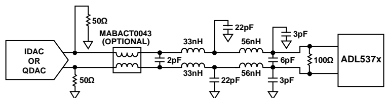
Figure 82. DAC Modulator Interface with Fifth-Order, Low Pass Filter
