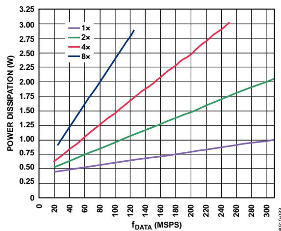
Figure 84. Total Power Dissipation vs. f_{\text{DATA}} with Fine Modulation, PLL, and Inverse Sinc Filter Disabled
