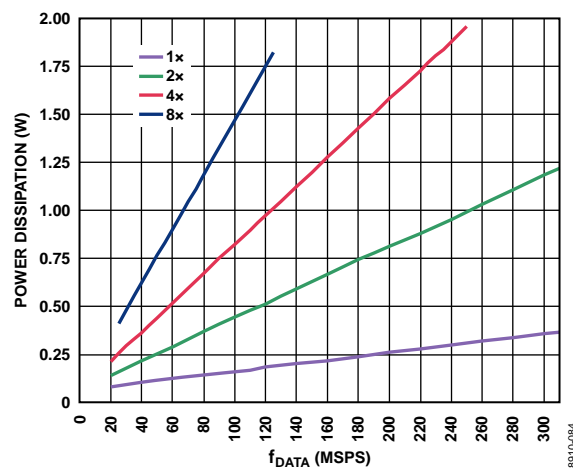
Figure 85. DVDD18 Power Dissipation vs. f_{\text{DATA}} with Coarse Modulation, PLL, and Inverse Sinc Filter Disabled
