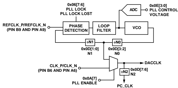
Figure 73. PLL Clock Multiplication Circuit
