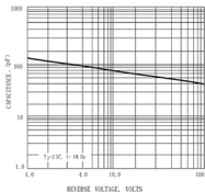
FIG. 3 - TYPICAL JUNCTION CAPACITANCE
