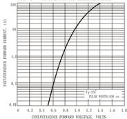
FIG. 4 - TYPICAL FORWARD CHARACTERISTICS
