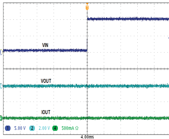
Power ON with Input Overvoltage
