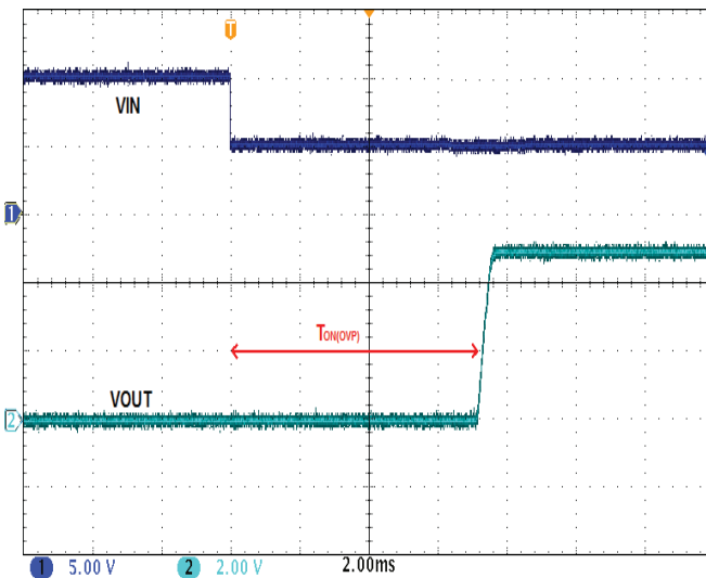
OVP Recovery Time
