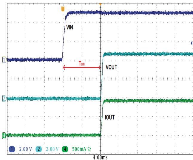
Normally Power ON
