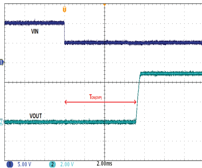
OVP Recovery Time
