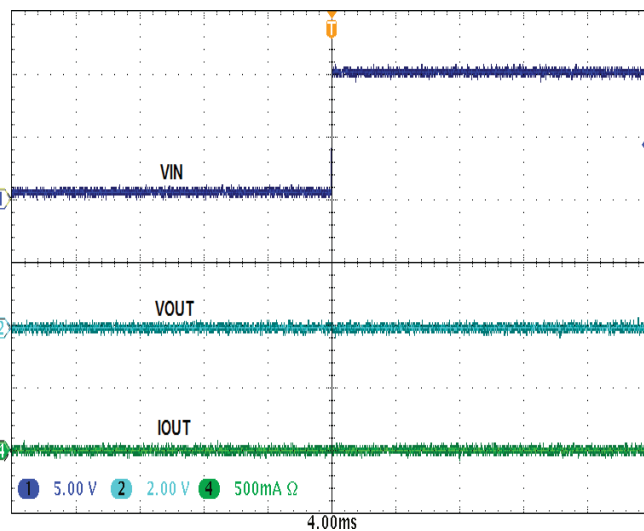
Power ON with Input Overtoltage
