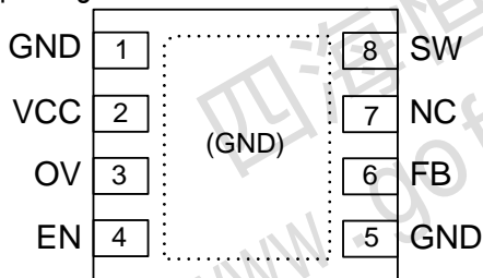
TDFN-8L (2*2)
