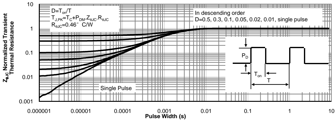
Figure 13: Normalized Maximum Transient Thermal Impedance for AOTF11N60(Note F)
