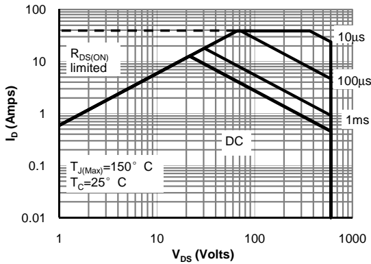
Figure 9: Maximum Forward Biased Safe Operating Area for AOTF11N60 (Note F)
