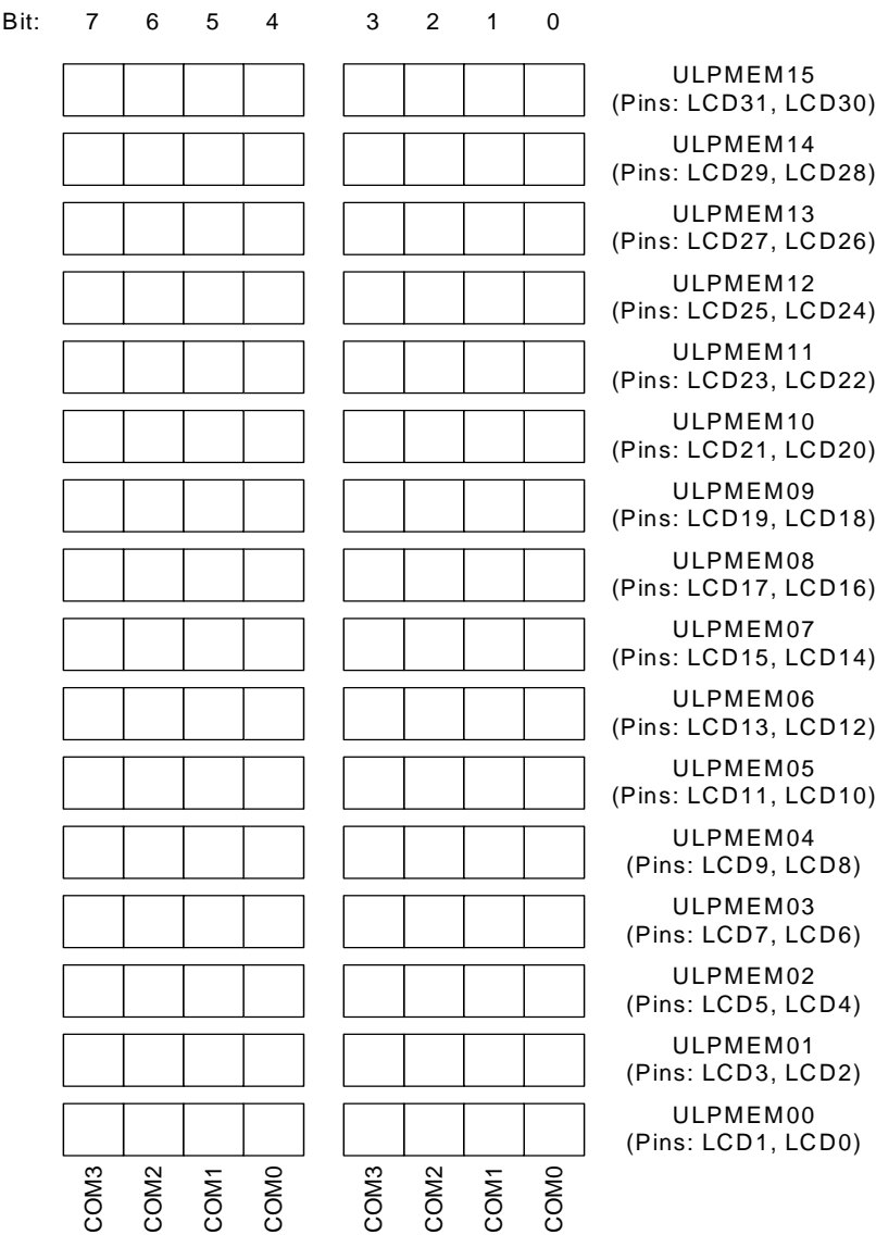
Figure 12.2. ULP Memory Map
