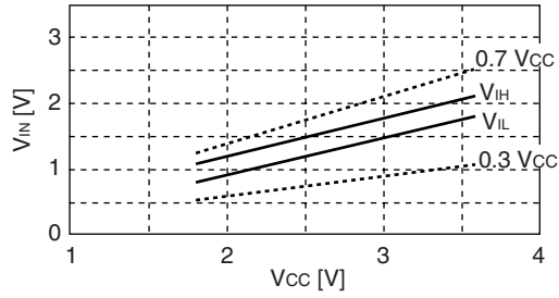
MB95F118AS/AW Hysteresis input characteristics of CMOS input level T_A = +25\text{ }^\circ\text{C}
