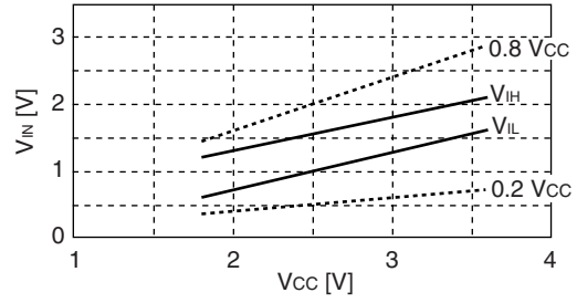
MB95116A Hysteresis input characteristics T_A = +25\text{ }^\circ\text{C}
