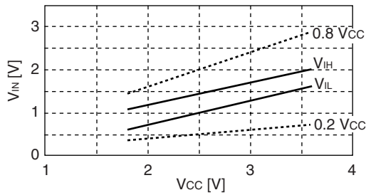
MB95F118AS/AW Hysteresis input characteristics T_A = +25\text{ }^\circ\text{C}
