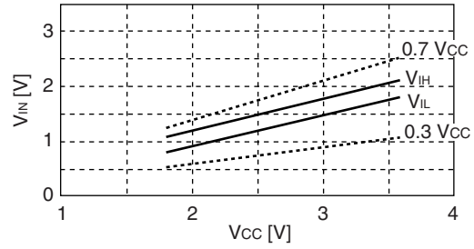
MB95116A Hysteresis input characteristics of CMOS input level T_A = +25\text{ }^\circ\text{C}
