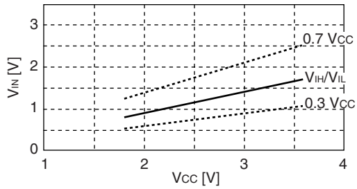
MB95F118AS/AW CMOS input characteristics T_A = +25\text{ }^\circ\text{C}
