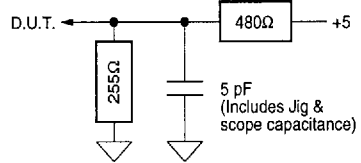
Figure 1b. Output Disable Timing Load
