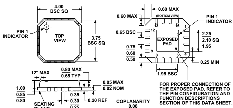
Figure 57. 16-Lead Lead Frame Chip Scale Package [LFCSP_VQ] 4 mm × 4 mm Body, Very Thin Quad (CP-16-4) Dimensions shown in millimeters
