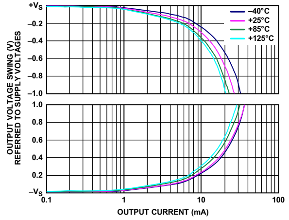
Figure 34. Instrumentation Amplifier Output Voltage Swing vs. Output Current, V_S = 5\text{ V}
