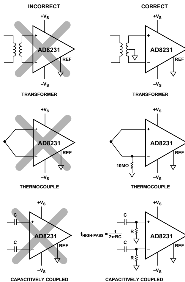
Figure 51. Creating an I_{\text{BIAS}} Path
