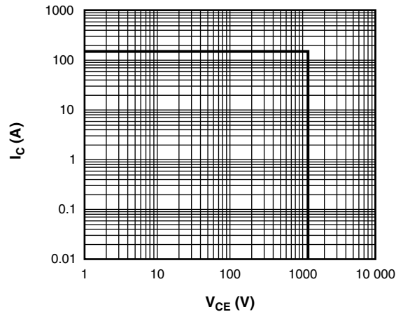
Fig. 2 - IGBT Reverse Bias SOA T_J = 150^\circ\text{C}, V_{GE} = 15 V
