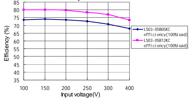
LS03-05BXXKC AC input rated load efficiency curve
