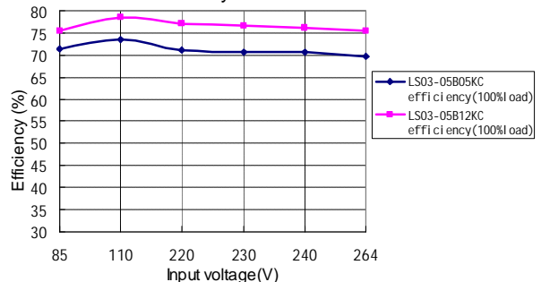
LS03-05BXXKC AC input rated load efficiency curve
