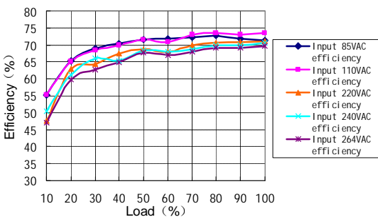
LS03-05BXXKC AC input efficiency curve
