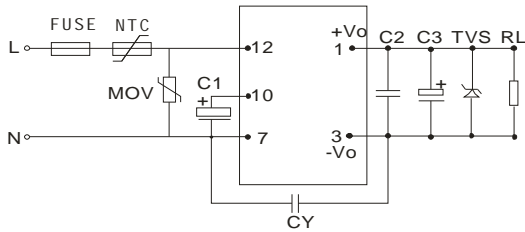
Figure 1: LS03-05BXXKC
