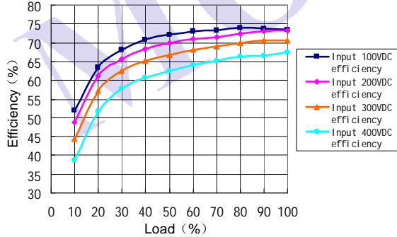
LS03-05BXXKC DC input efficiency curve
