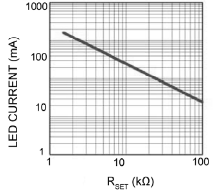
Six Parallel Channels Current vs. RSET
