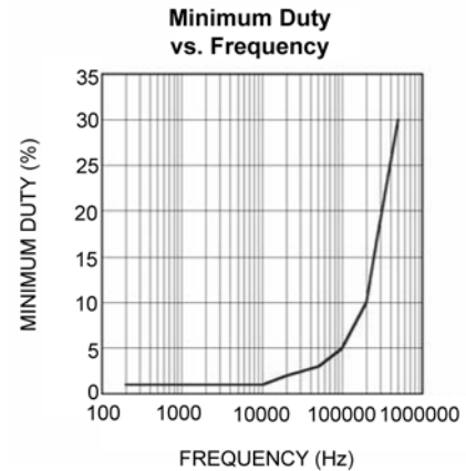
Figure 5. Minimum Duty Cycle for Varying PWM Frequency
